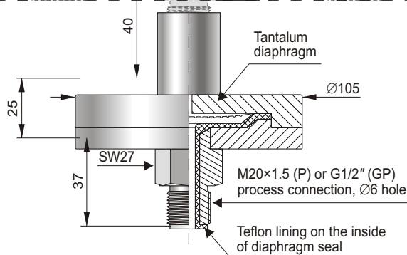
Version with M20x1,5 process connection
