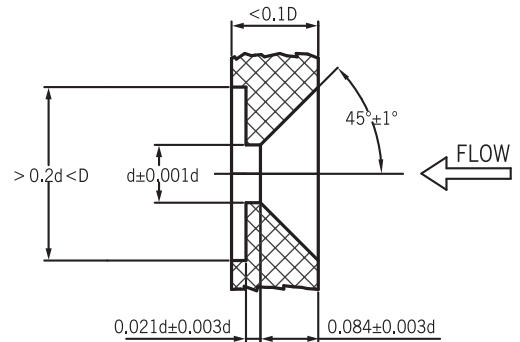
Conical Entrance Orifice Plate
