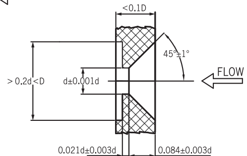
Conical Entrance Orifice Plate
