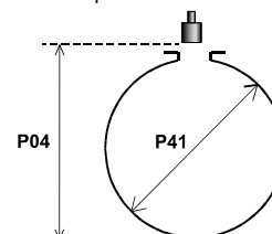
Spherical tank
