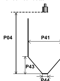
Standing cylindrical tank with conical bottom
