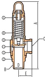
N9SP TYPE Sealing 1/2"~2"
