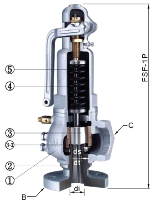
FSF-1P Lever 1"~2"
