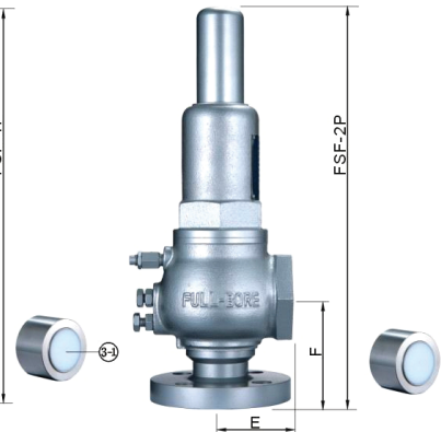
FSF-2P Sealing 1"~2"
