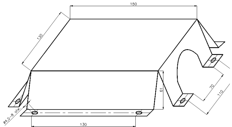
Pic.1 Float seal
