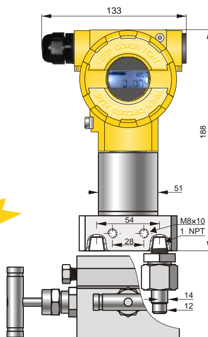
APR-2000GALW Industrial Version, C type process connector to be mounted along with a valve manifold
