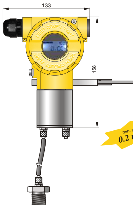
APR-2000GALW Economic Version, process connection with terminal connecting to 6 pipe (PCV type)
