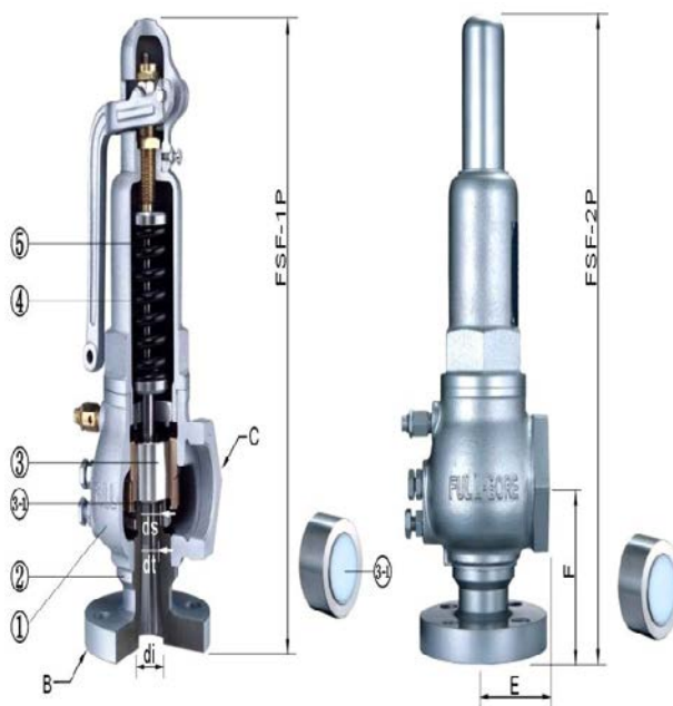
Van an toàn FSF-1p/FSF-2p
