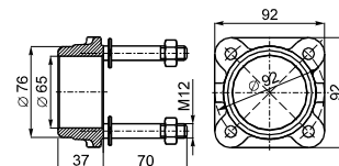
Counter flange for MFF-111 , 121 version with tester
