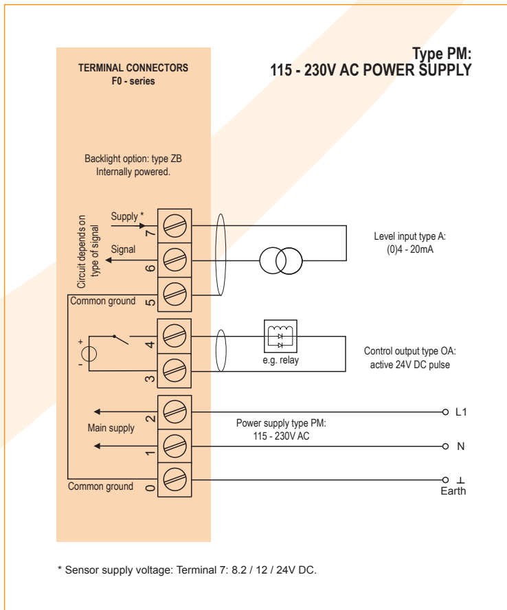
Typical wiring diagram F074-A-OA-PM-ZB
