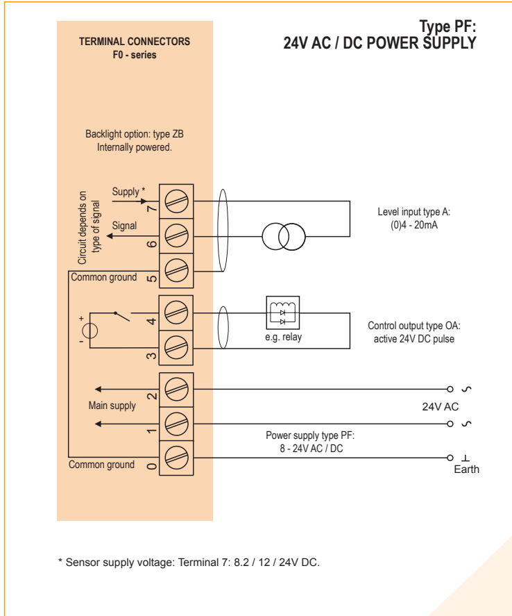
Typical wiring diagram F074-A-OA-PF-ZB
