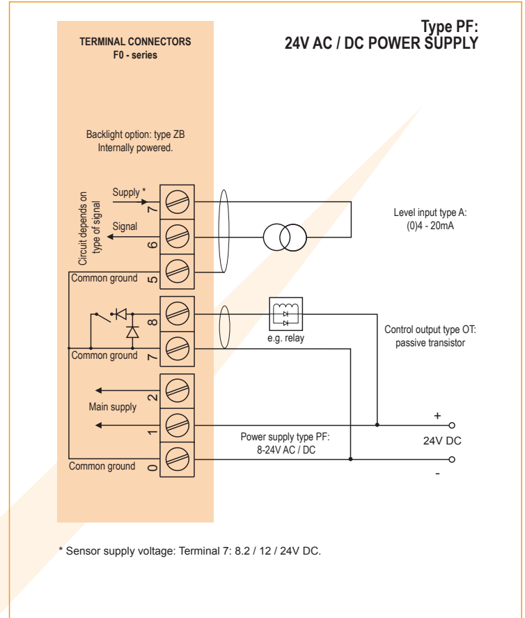
Typical wiring diagram F074-A-OT-PF-ZB
