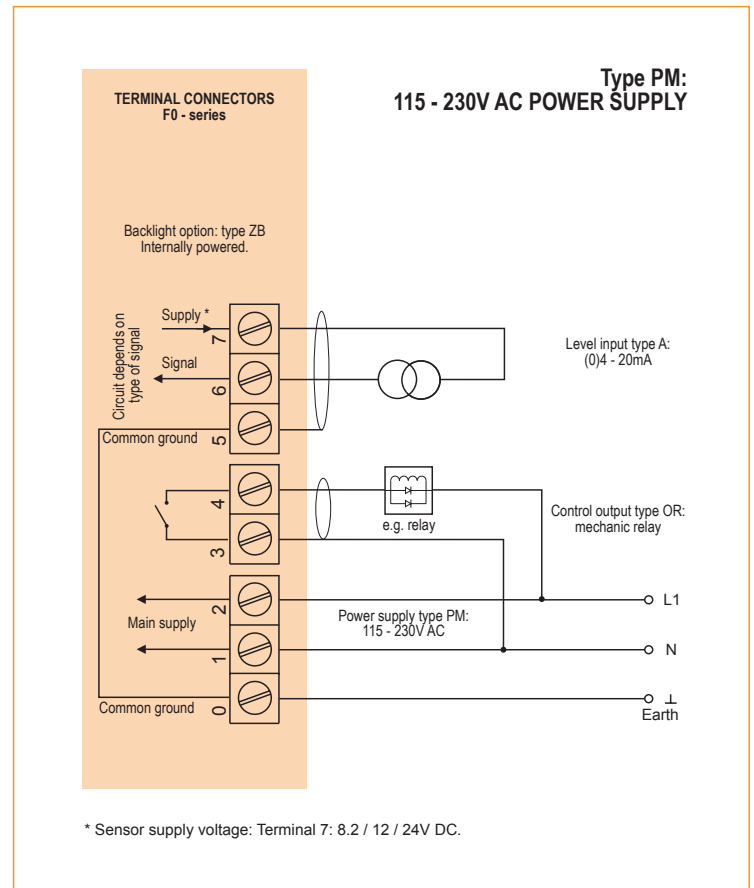
Typical wiring diagram F074-A-OR-PM-ZB
